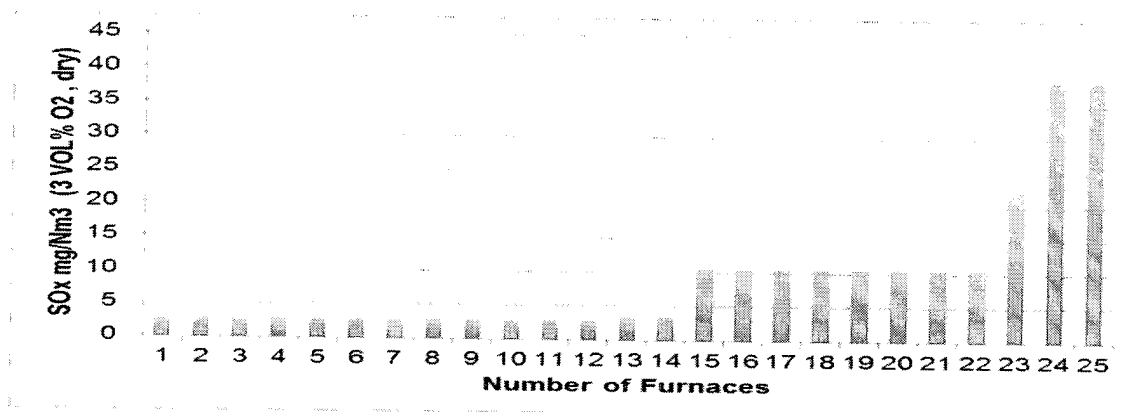
Figure 11: furnace sulfur emissions during normal operation.
