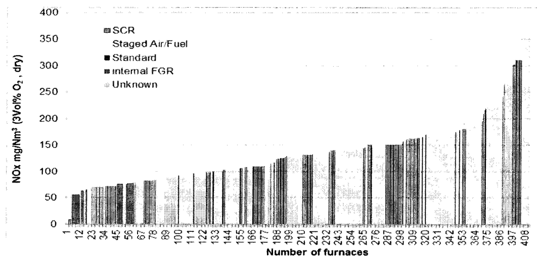
Figure 6: Steam cracker furnace NOx emissions categorized per NOx abatement
