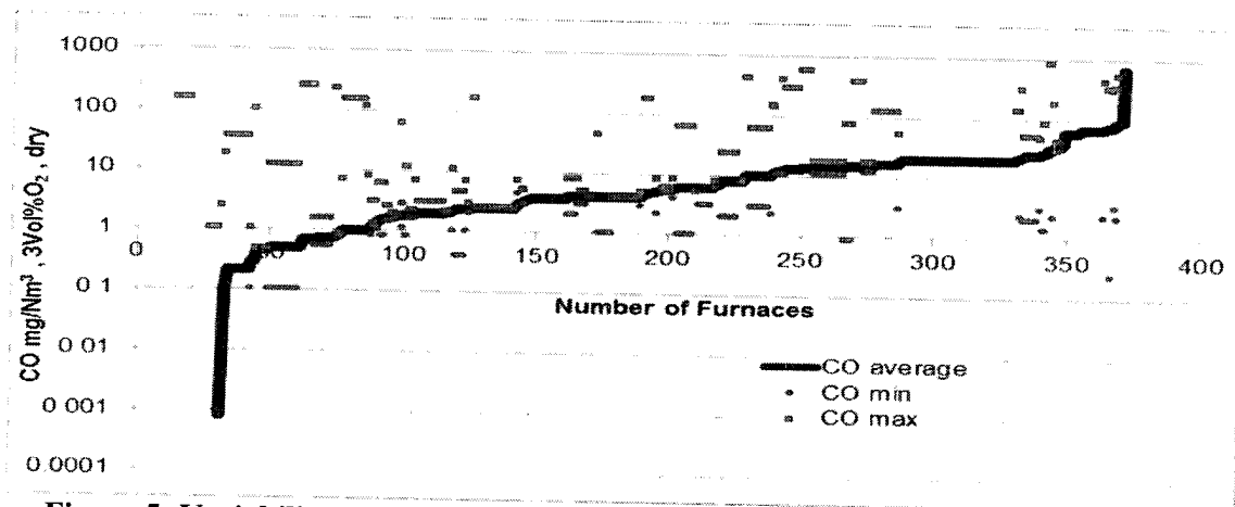
Figure 5: Variability of CO emissions of all furnaces
